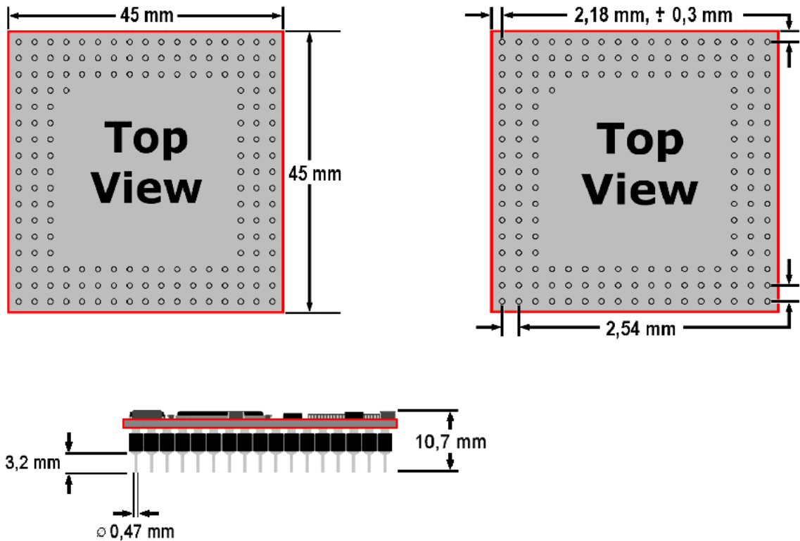
Figure 1: PNP/1110 Mechanical Dimensions
